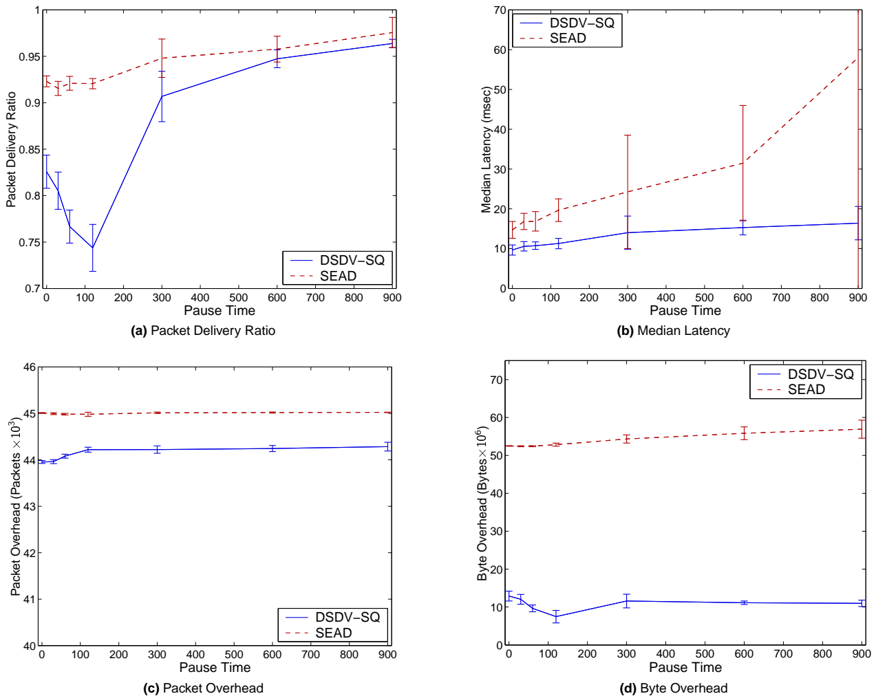
Figure 1: SEAD performance evaluation results (average over 65 runs)
