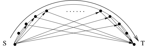
Figure 3: The performance of max-min path can be very bad. In this example, each node except for the source S has the power 20 + \epsilon , and the weight of each edge on the arc is 1. The weight of each straight edge is 2. Let the power of the source be \infty . The network can send 20 messages from S to T according to max-min strategy by taking the edges on the arc (see the arc on the top). But the optimal number of messages follows the straight edges with black arrows is 10(n - 4) where n is the number of nodes.
