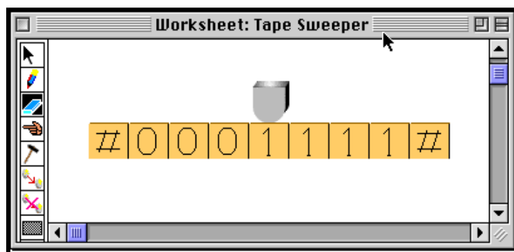
Figure 15: The Turing machine head after moving one position to the right.
