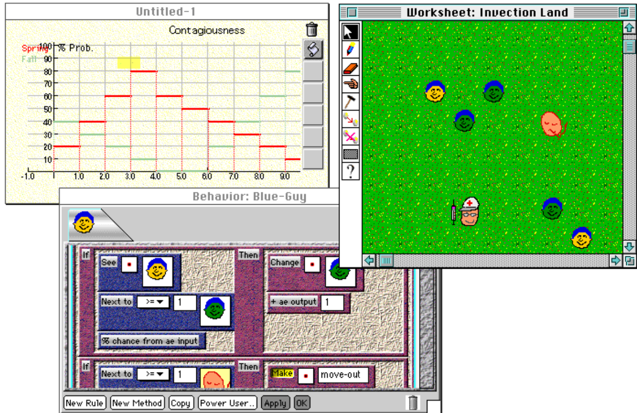
Figure 34: SimCalc (top left) Combined with AgentSheets
