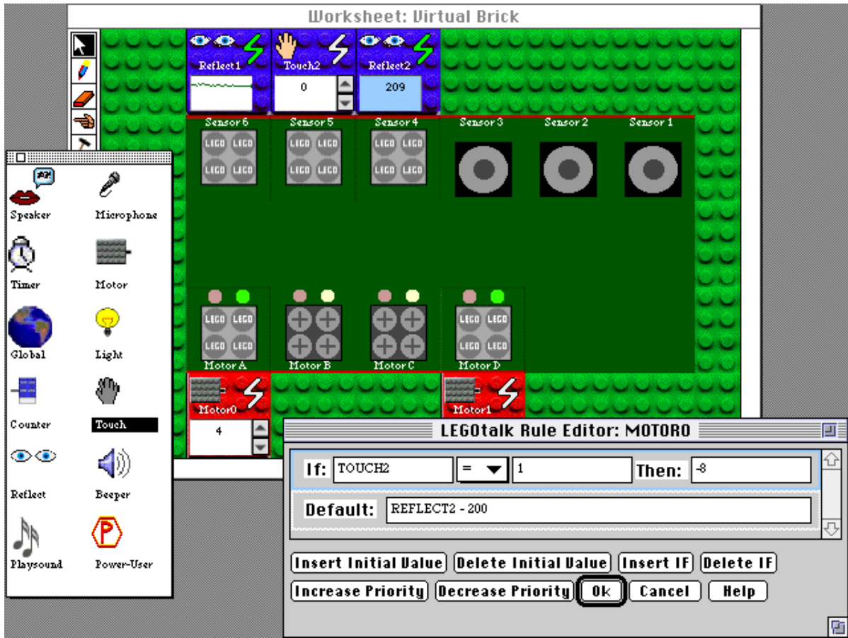
Figure 18: The LEGOsheets environment
