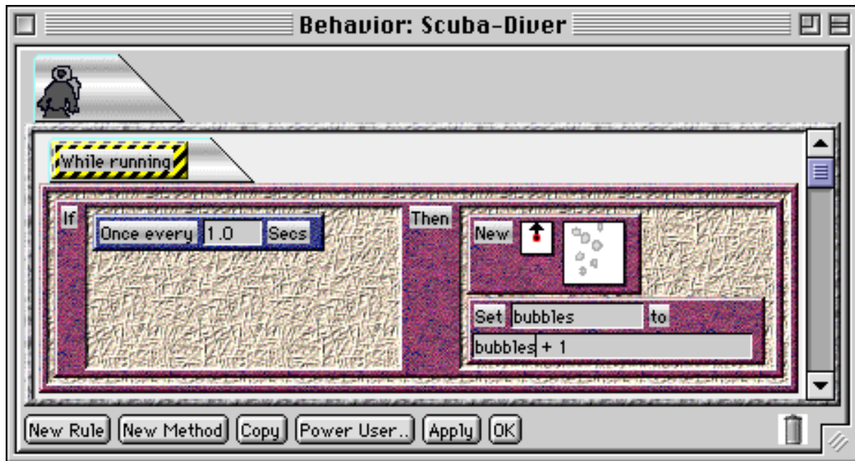
Figure 32: Modified diver behavior creating a new bubble every second and counting the number of bubbles.
