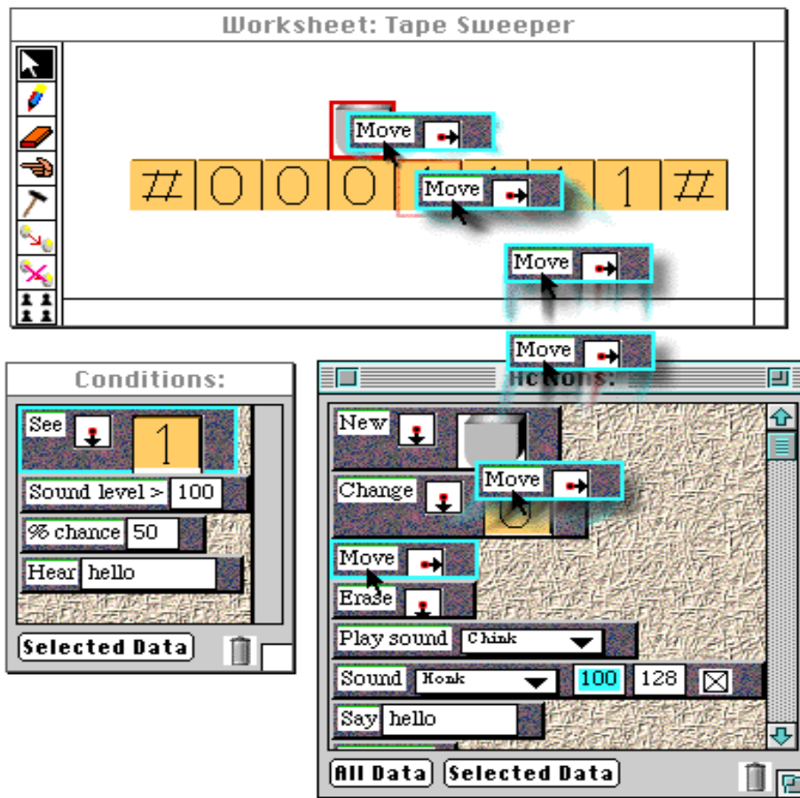
Figure 14: Commands can be dragged and dropped onto agents to explore their function and to modify agents
