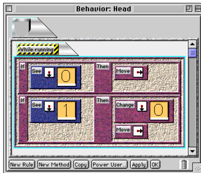
Figure 16: Visual AgenTalk Rules for the Tape Head.
