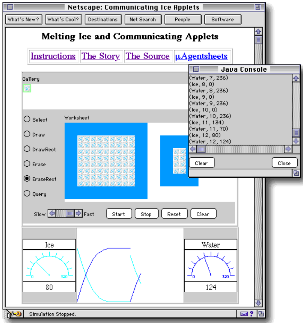
Figure 35: The Melting Ice Applet Combined with other Applets
