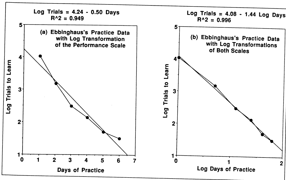
Fig. 3. The practice data from Figure 1b with (a) the performance measure transformed according to logarithmic function and (b) both performance measures transformed according to a logarithmic function.
