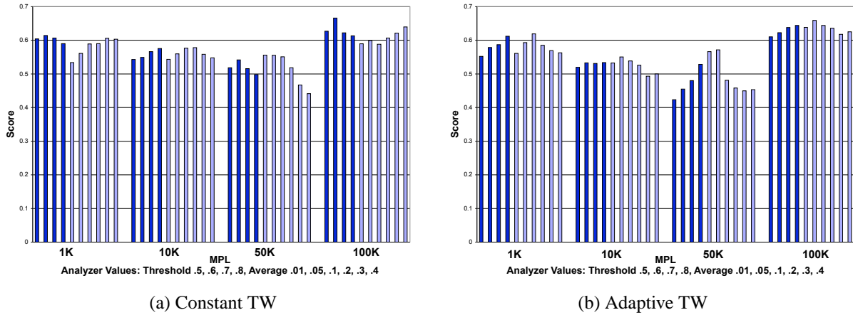
Figure 6: The average of best scores across all benchmarks for the Constant TW (a) and the Adaptive TW (b). Each chart is grouped into four sets of bars, one for each MPL value. Each MPL category has ten analyzers corresponding to (from left to right) the four Threshold analyzers (darker bars) with increasing threshold (0.5, 0.6, 0.7, 0.8) and the six Average analyzers (lighter bars) with increasing deltas (0.01, 0.05, 0.1, 0.2, 0.3, 0.4).
