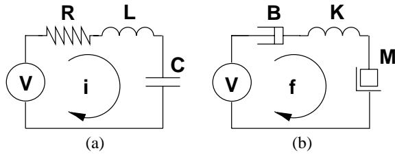
Figure 2: Two systems that are described by the same GPN model: (a) a series RLC circuit (b) a mass-spring-damper system. \mathbf{V} is a voltage source in (a) and is a velocity source in (b).
